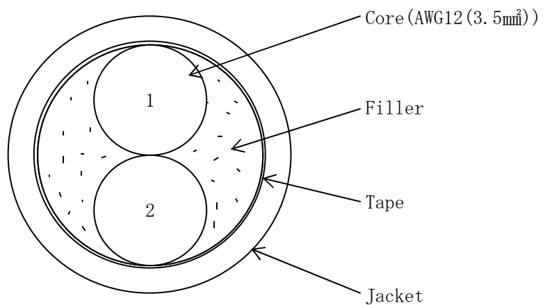
Cross-Section of Cable
